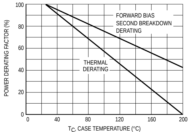
Figure 14. Power Derating
