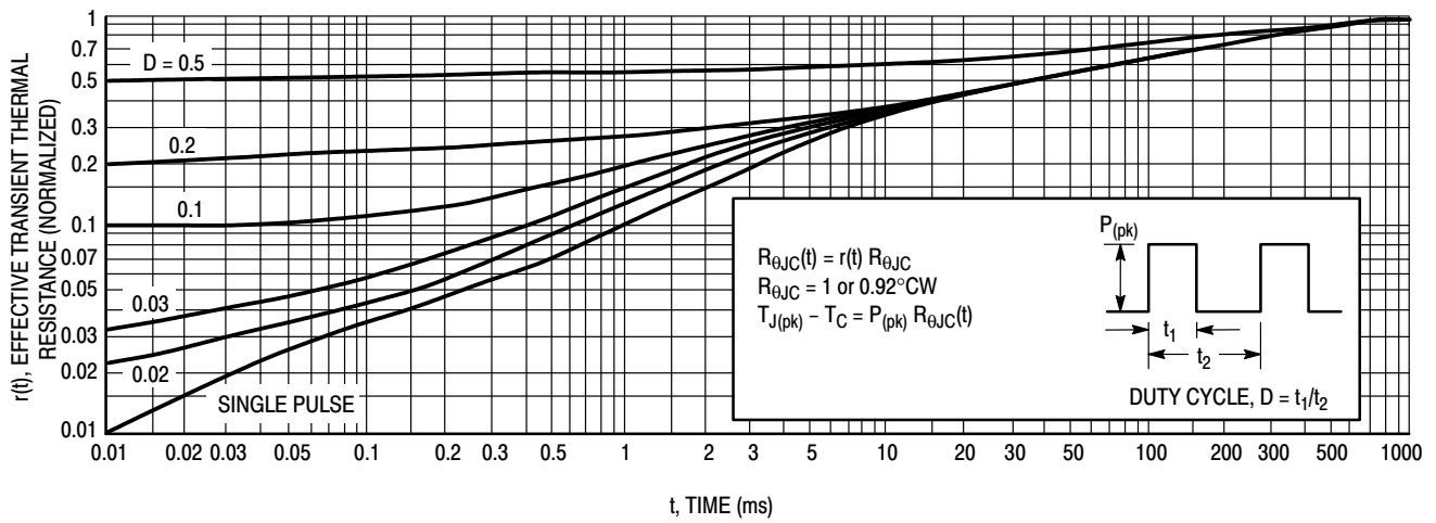
Figure 18. Thermal Response
