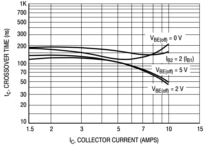
Figure 7. Crossover Time
