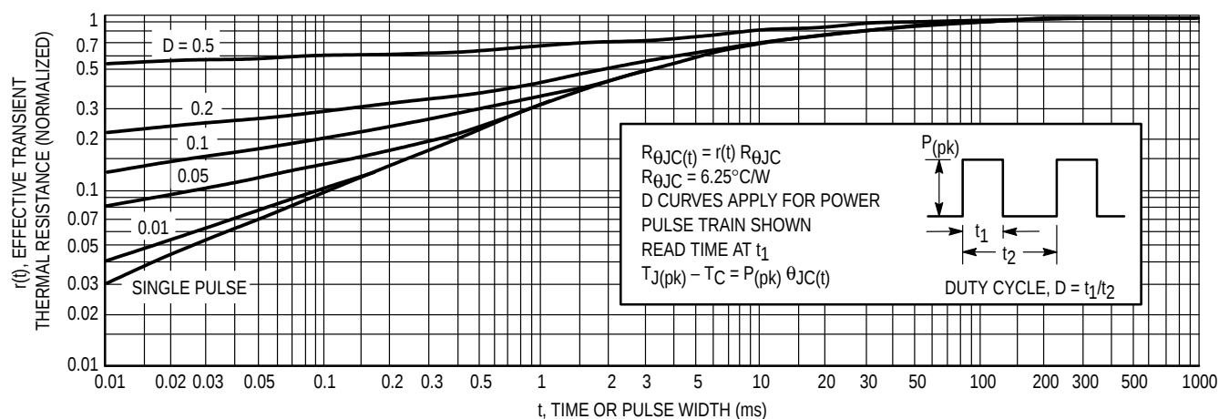
Figure 3. Thermal Response
