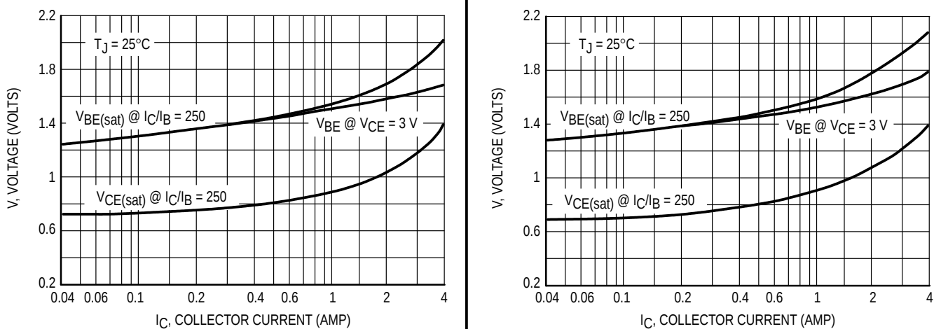
Figure 9. "On Voltages"
