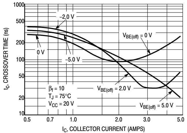
Figure 12. Crossover Time
