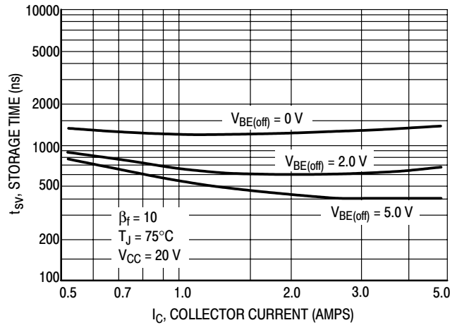
Figure 8. Storage Time
