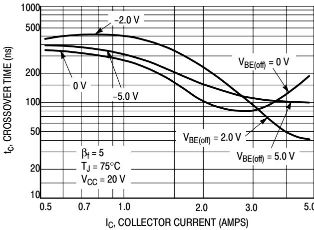
Figure 11. Crossover Time
