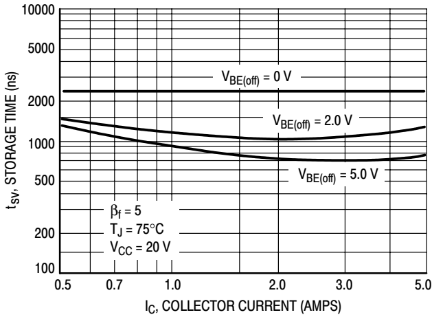
Figure 7. Storage Time
