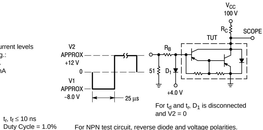
Figure 2. Switching Times Test Circuit
