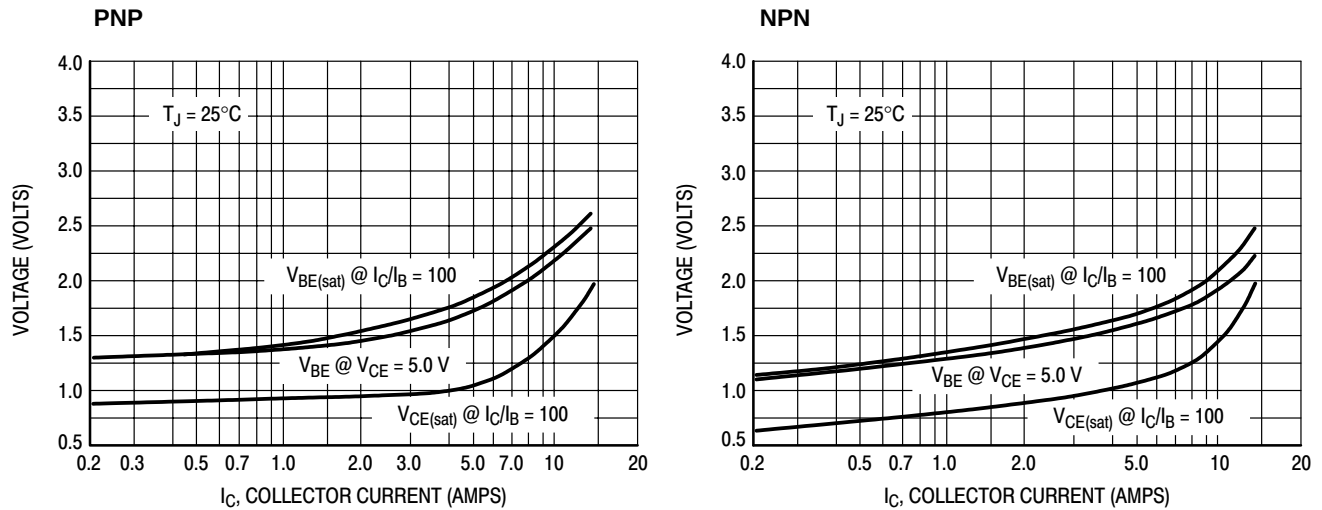
Figure 8. "On" Voltages
