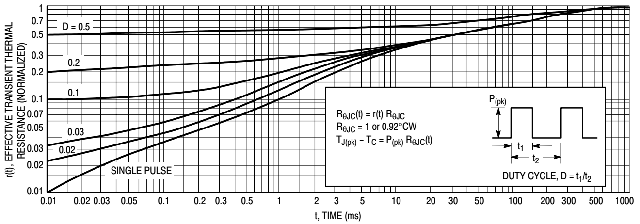
Figure 18. Thermal Response
