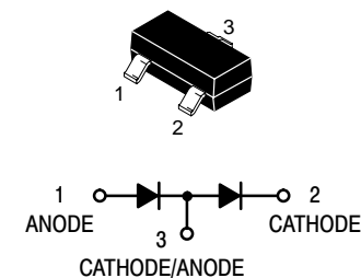
MMBD352LT1 CASE 318-08, STYLE 11 SOT-23 (TO-236AB)
