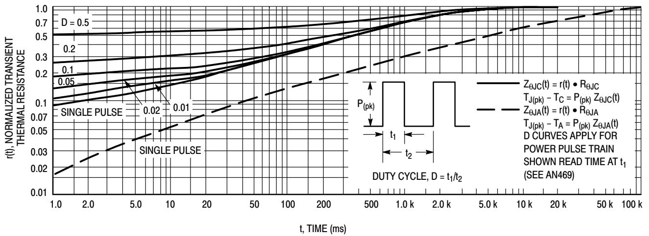
Figure 10. Thermal Response
