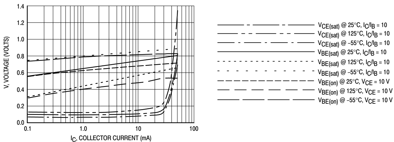
Figure 4. "ON" Voltages
