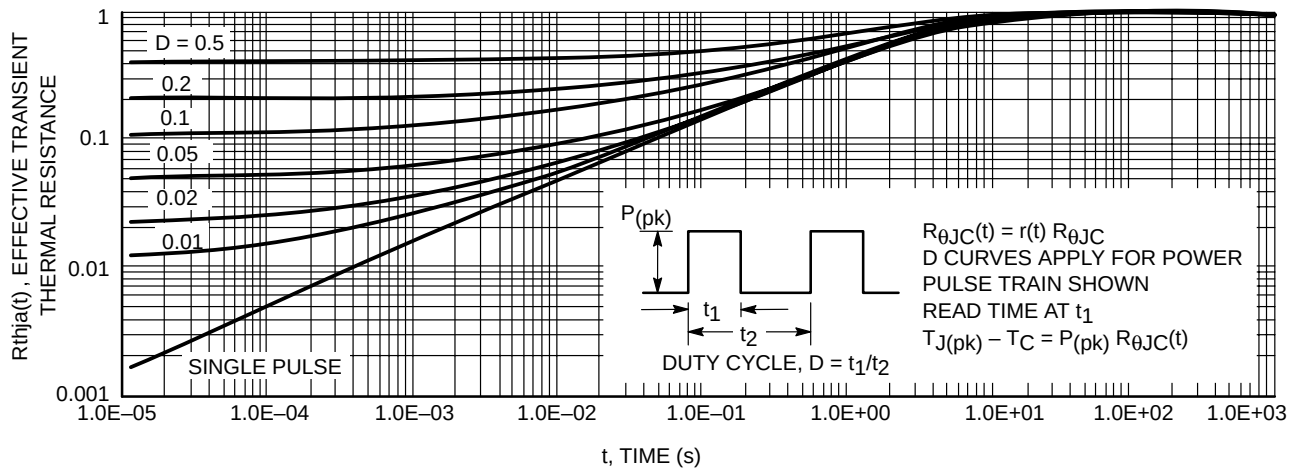
Figure 13. Thermal Response
