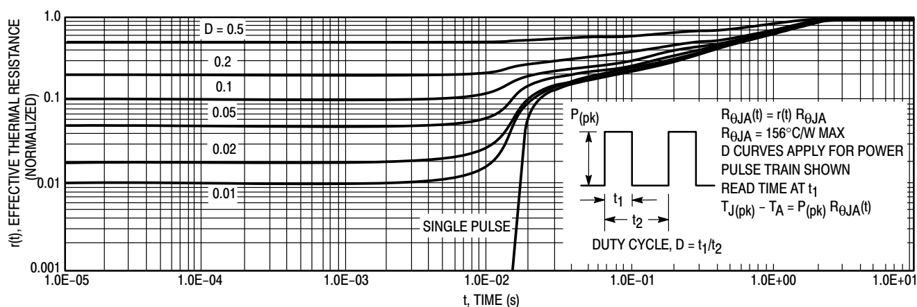
Figure 8. Thermal Response
