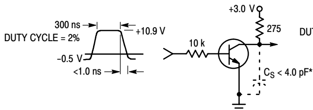
Figure 1. Turn-On Time
