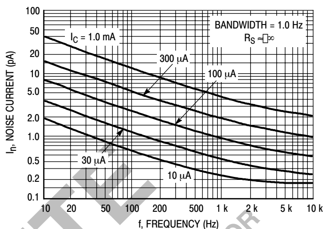
Figure 4. Noise Current
