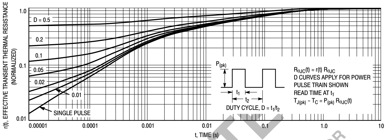
Figure 14. Thermal Response
