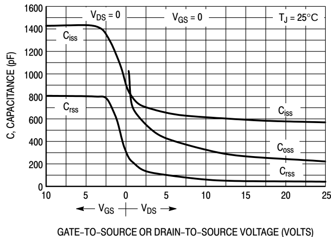
Figure 7. Capacitance Variation
