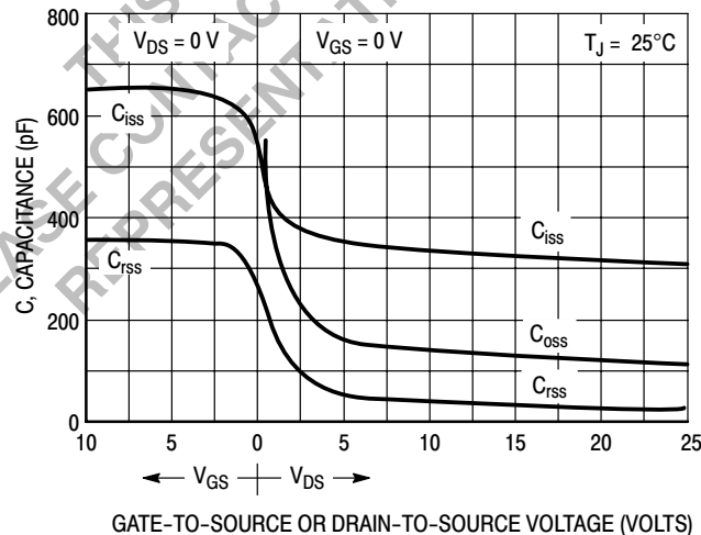
Figure 7. Capacitance Variation
