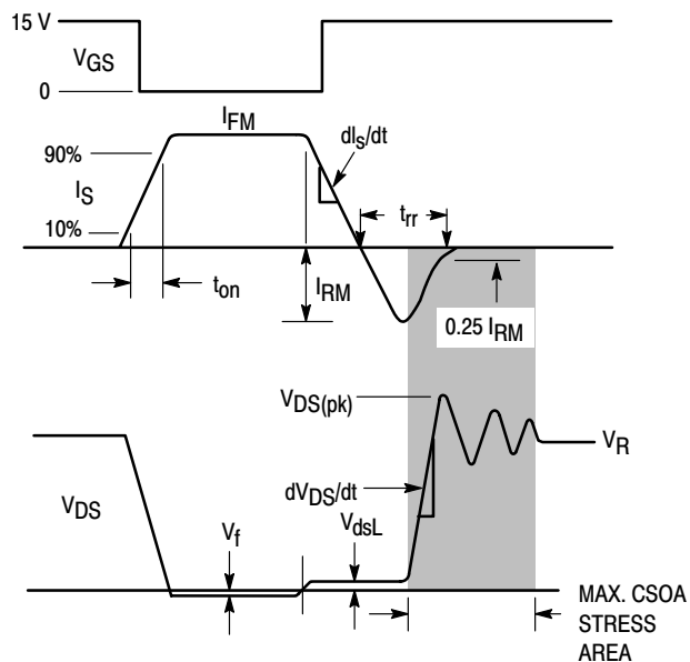
Figure 11. Commutating Waveforms
