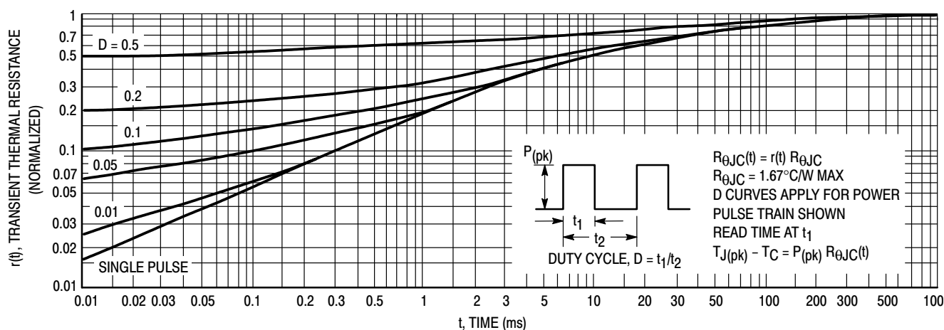
Figure 10. Thermal Response
