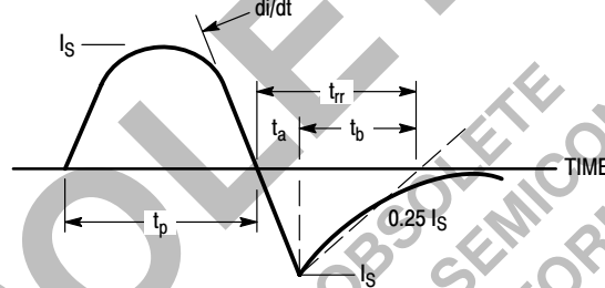
Figure 15. Diode Reverse Recovery Waveform
