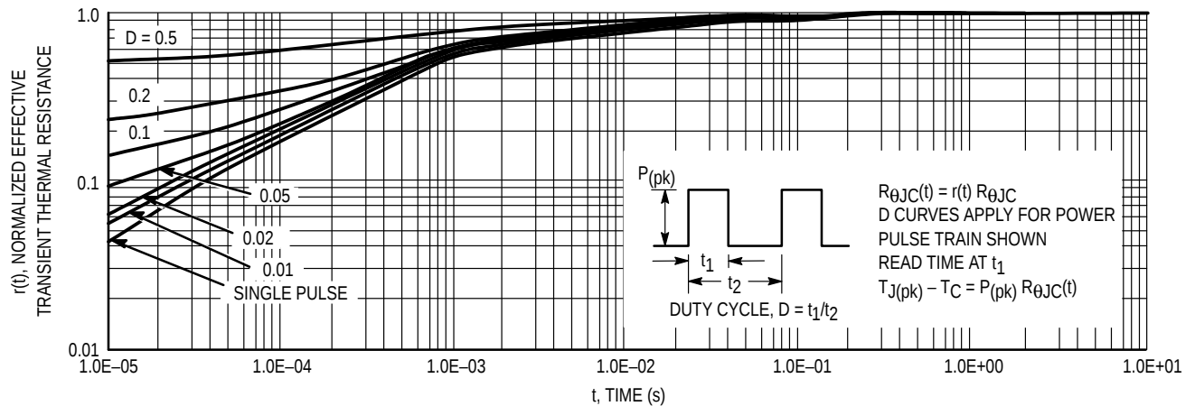
Figure 13. Thermal Response
