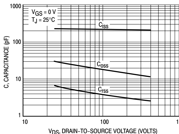
Figure 7b. High Voltage Capacitance Variation
