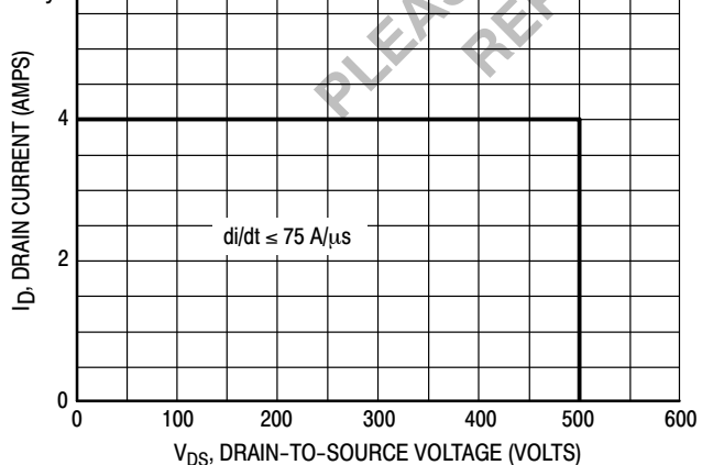
Figure 13. Commutating Safe Operating Area (CSOA)
