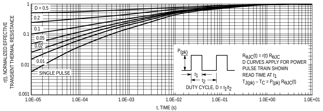
Figure 14. Thermal Response
