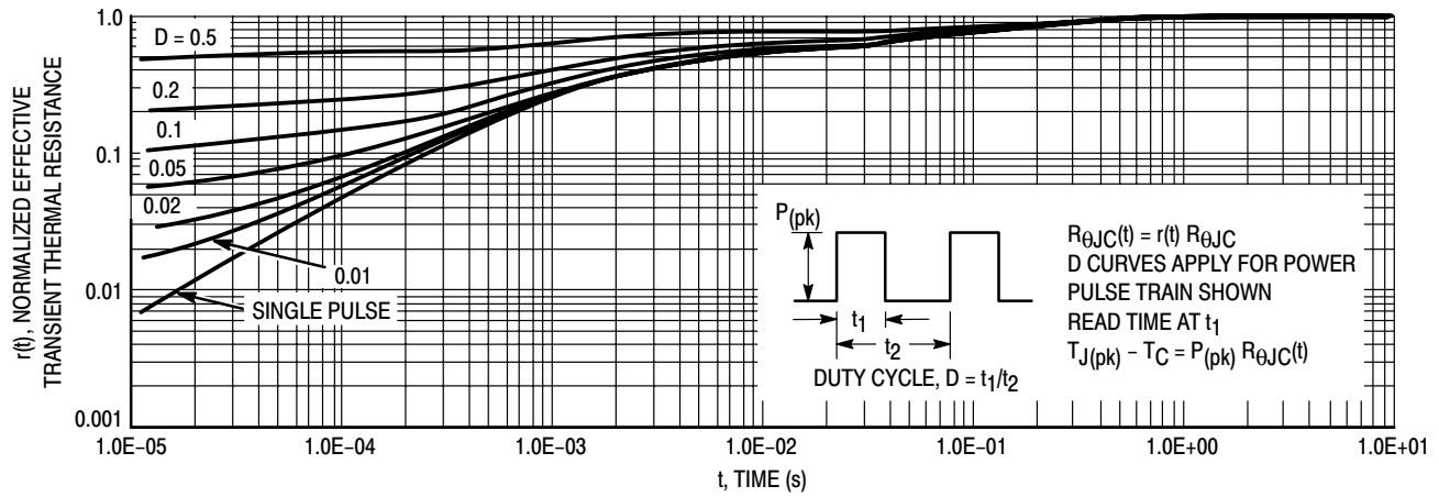
Figure 12. Thermal Response
