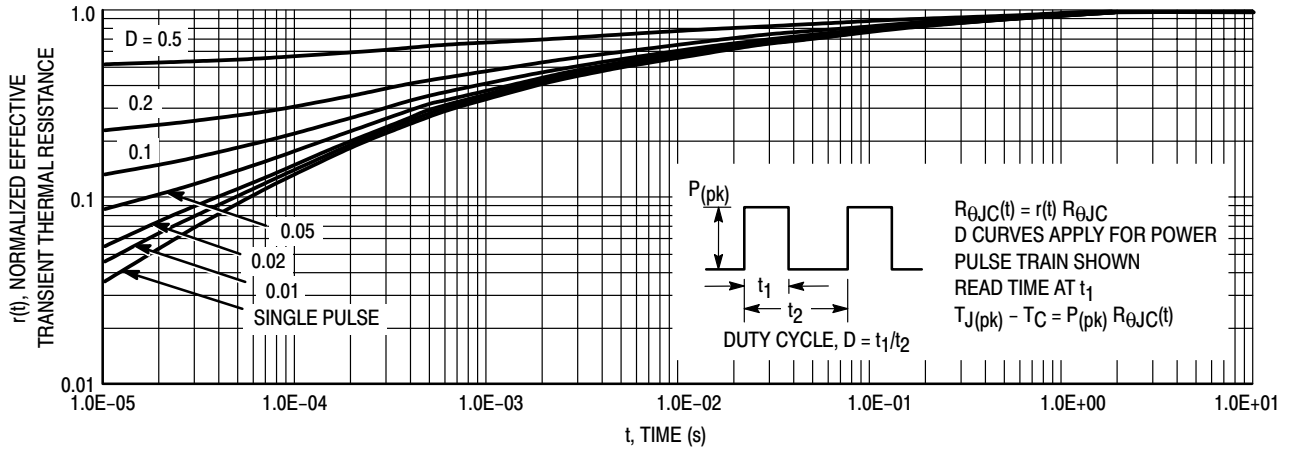
Figure 13. Thermal Response
