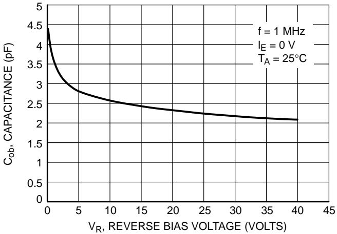
Figure 24. Output Capacitance
