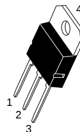
TO-218AC CASE 340D STYLE 2
