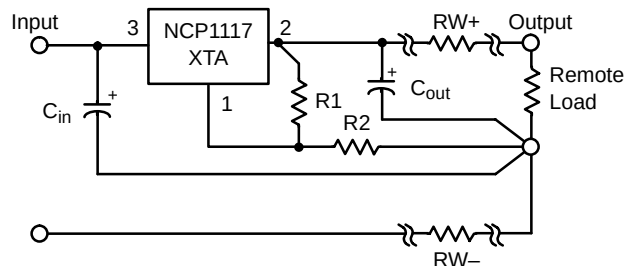
Figure 23. Load Sensing
