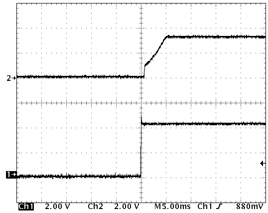
( V_{IN} = 4.3\text{ V} , V_{OUT} = 3.3\text{ V} , C_{SS} = 100\text{ pF} , No load) Upper Trace: Output Voltage, 2.0 V/Div. Lower Trace: EN Pin Waveform, 2.0 V/Div. Time Scale: 5.0 ms/Div.
