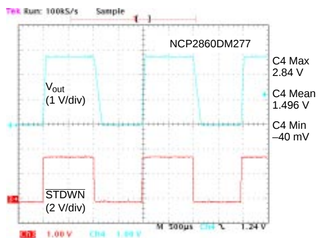
Figure 13. Shutdown/Power-Up ( V_{in} = V_{out} + 0.5 V, I_{load} = 50 mA)
