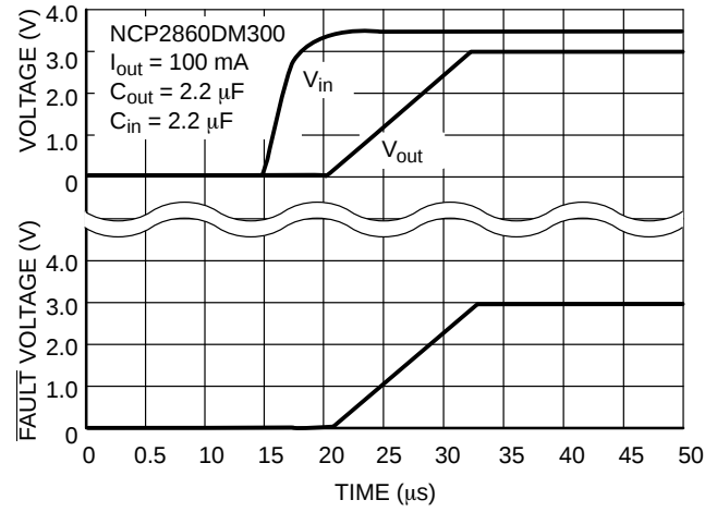
Figure 16. Power-Up Response
