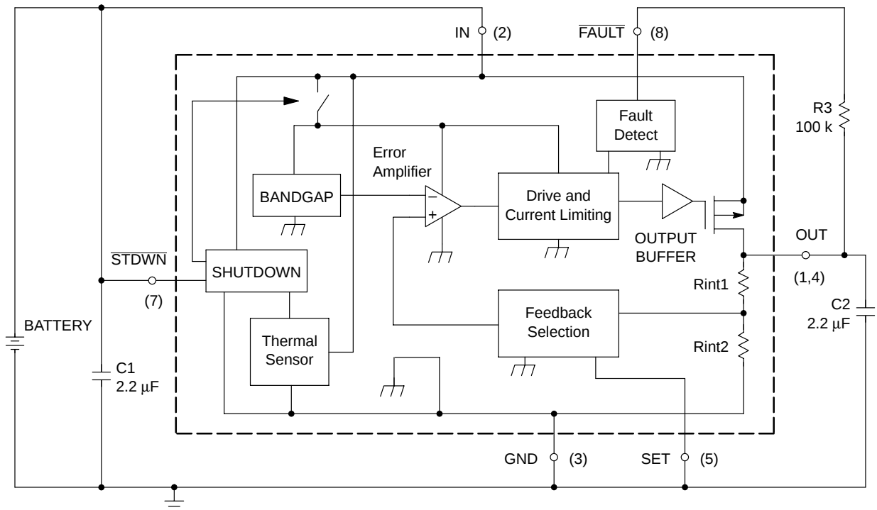
Figure 19. Application for 2.77 V Output Voltage
