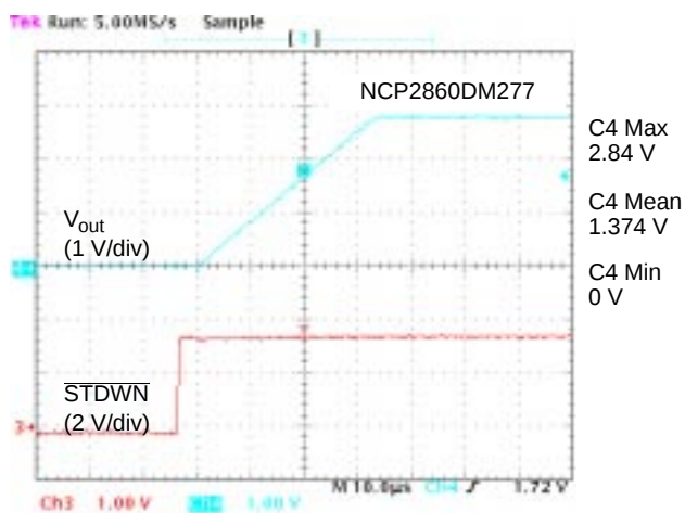
Figure 14. Shutdown/Power-Up ( V_{in} = V_{out} + 0.5 V, I_{load} = 0 mA)
