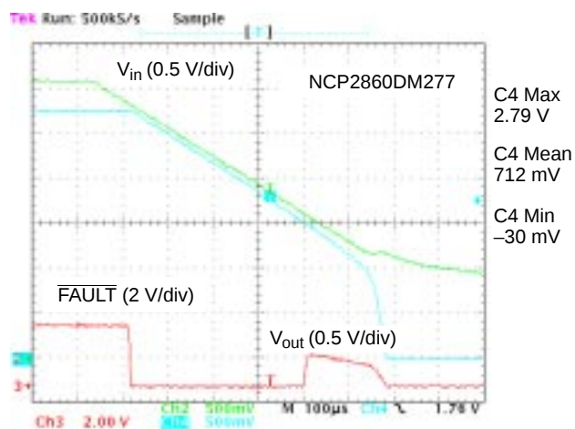
Figure 11. Power-Down Response ( I_{load} = 100 mA)
