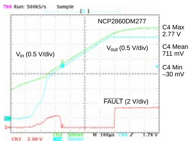
Figure 12. Power-Up Response ( I_{load} = 100 mA)
