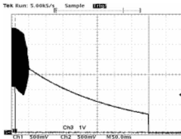
Figure 30. Turning Off Time - V_p = 5 V
