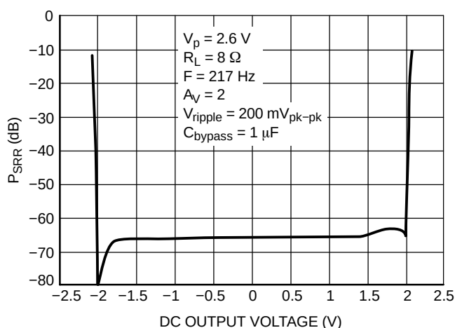
Figure 28. PSRR @ DC Output Voltage
