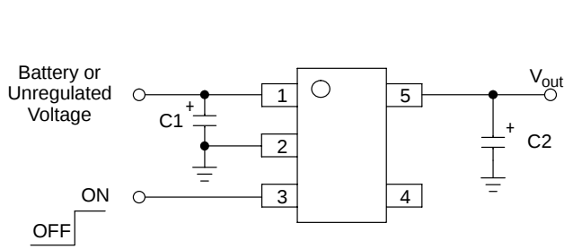
Figure 27. Typical Application Circuit
