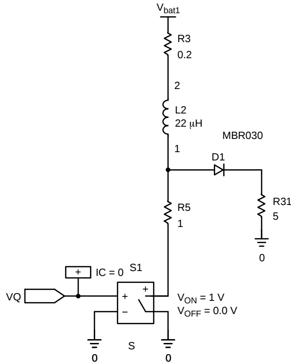
Figure 2. Typical Boost Topology Converter
