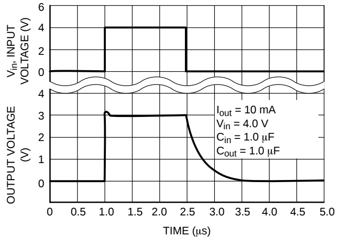
Figure 11. Turn-on Response
