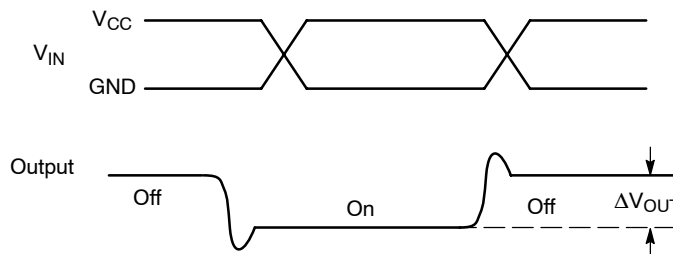
Figure 7. Charge Injection: (Q)
