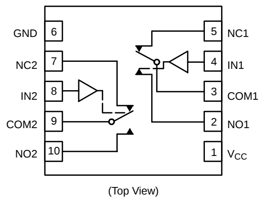
Figure 1. Pin Connections and Logic Diagram (QFN-10 and Micro10)
