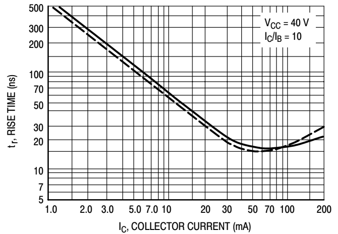
Figure 5. Rise Time
