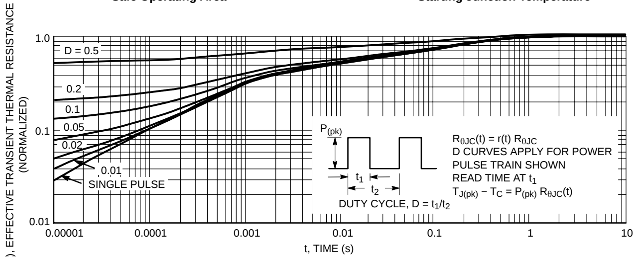
Figure 13. Thermal Response
