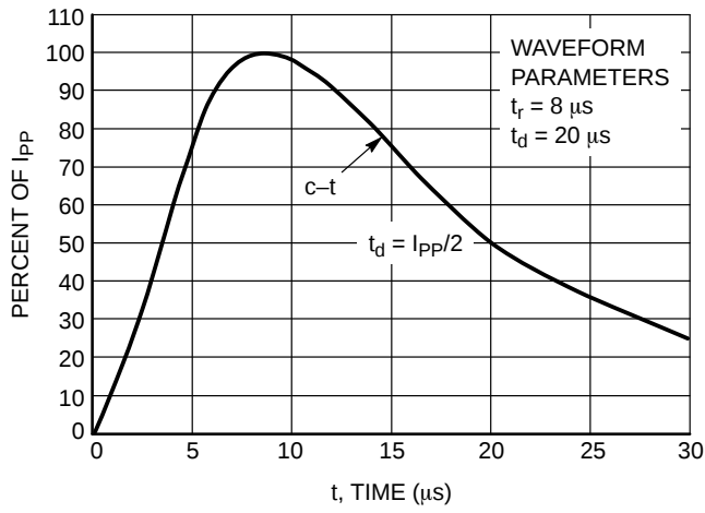
Figure 3. Pulse Waveform
