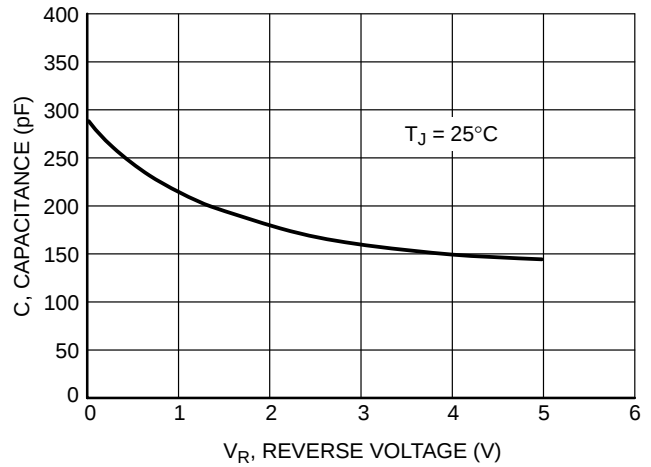
Figure 6. Typical Capacitance
