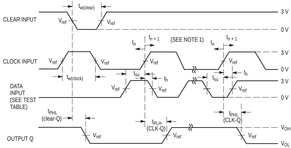
AC WAVEFORMS
