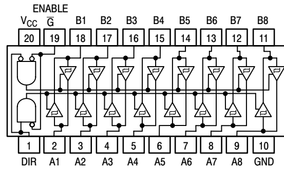
Figure 2. SN74LS641 SN74LS645
