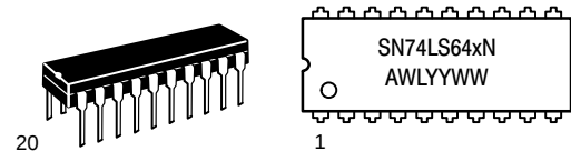
PDIP–20 N SUFFIX CASE 738
