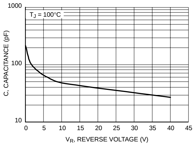
Figure 7. Capacitance
