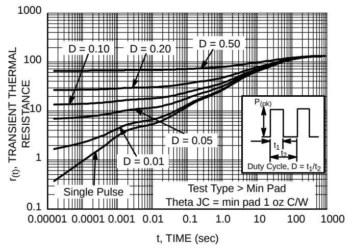
Figure 8. Thermal Response
