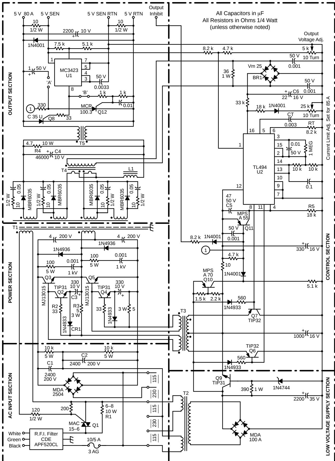
Figure 3. 400 Watt Switchmode Power Supply
