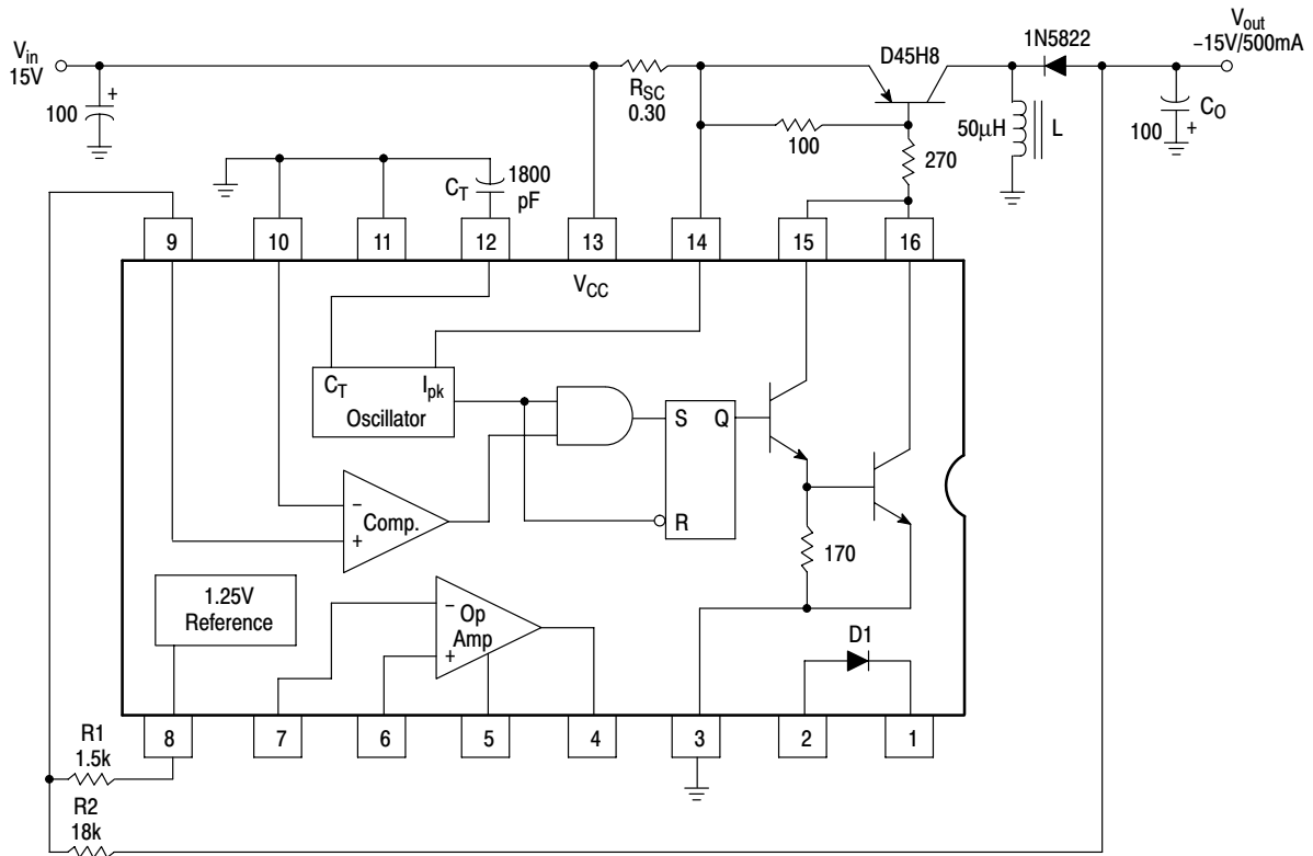
Figure 8. Inverting Converter
