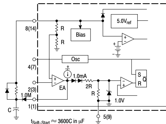
Figure 24. Soft-Start Circuit
