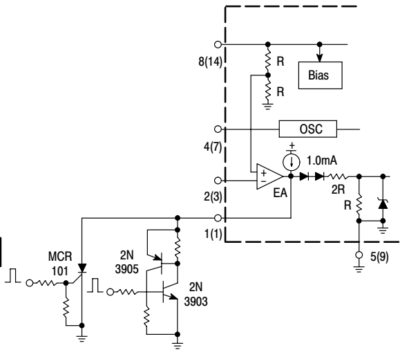
Figure 26. Bipolar Transistor Drive
