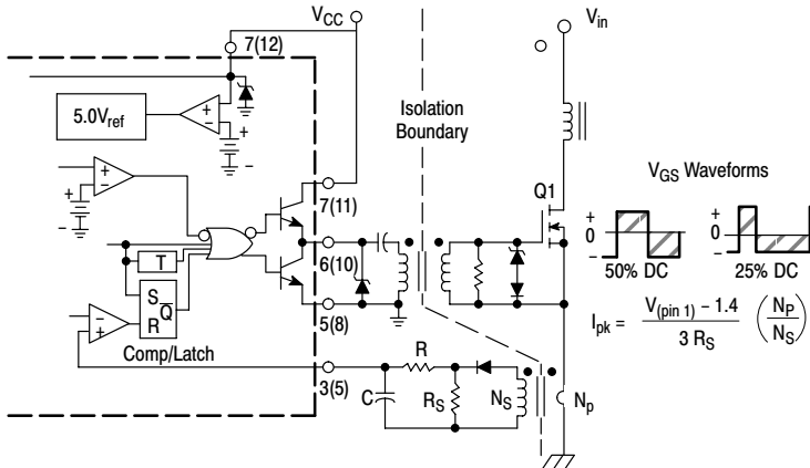
Figure 27. Isolated MOSFET Drive
