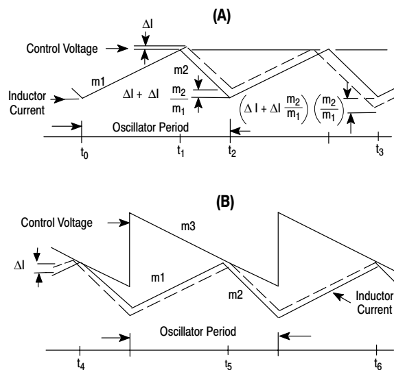
Figure 20. Continuous Current Waveforms
