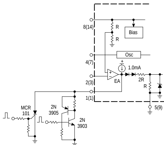
Figure 27. Latched Shutdown
