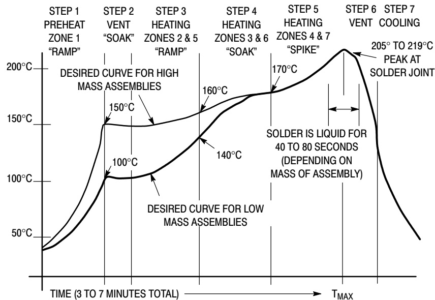
Figure 10. Typical Solder Heating Profile
