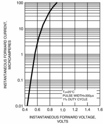
FIG. 4 - TYPICAL INSTANTANEOUS FORWARD CHARACTERISTICS
