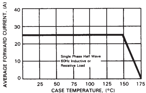
FIG. 3 - TYPICAL FORWARD CURRENT DERATING CURVE
