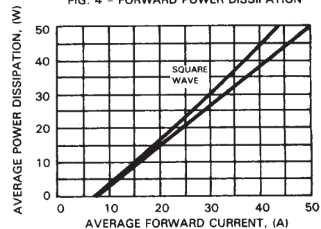
FIG. 4 - FORWARD POWER DISSIPATION
